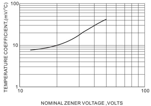
Fig.2 TEMPERATURE COEFFICIENTS
