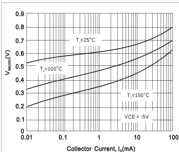
Fig.2- TYPICAL V_{BE(ON)} vs. Collector Current
